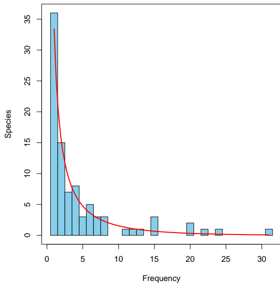
Figure 3: Fisher’s log-series fitted to one randomly selected site (26).
