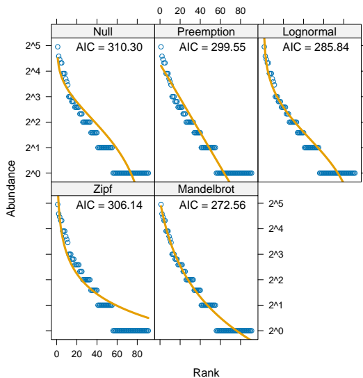
Figure 4: Ranked abundance distribution models for a random plot (no. 26). The best model has the lowest AIC.
