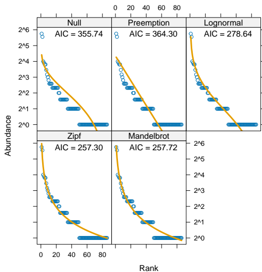
Figure 4: Ranked abundance distribution models for a random plot (no. 29). The best model has the lowest AIC.
