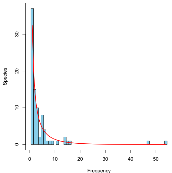
Figure 3: Fisher’s log-series fitted to one randomly selected site (29).
